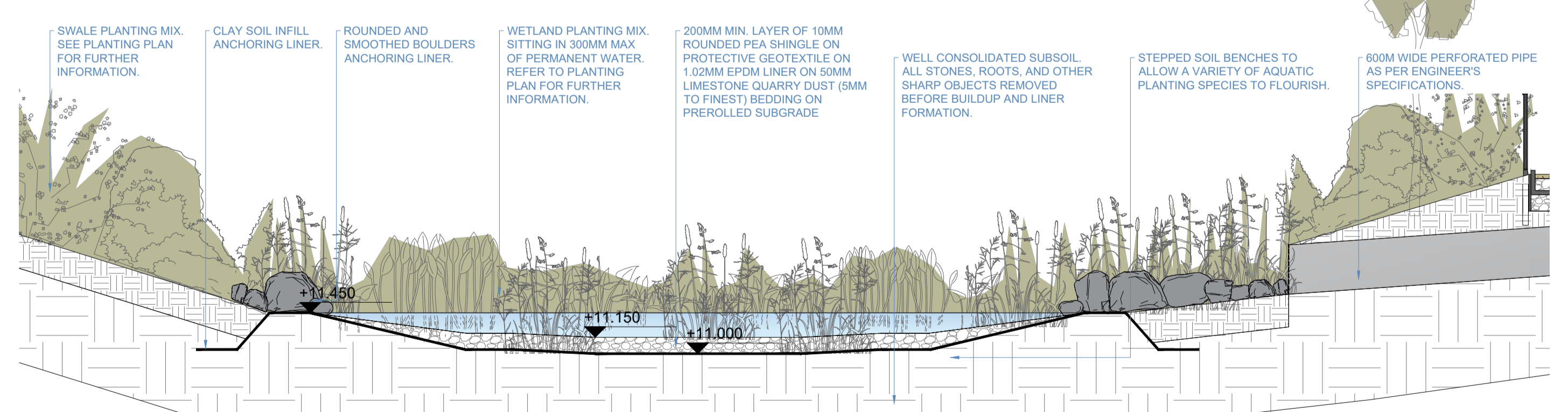
DETAIL W02 - WETLAND DETAIL SCALE : 1:50 / A1
