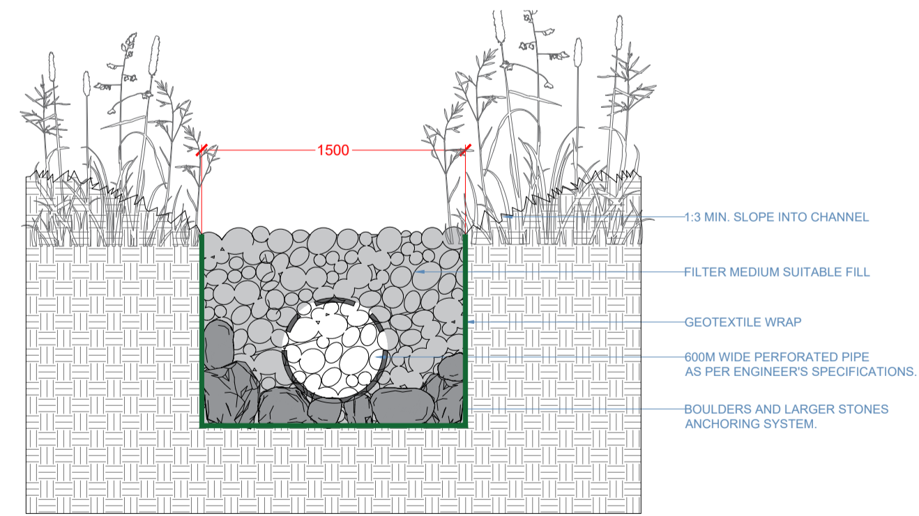
DETAIL W01 - CASCADING SWALE CHANNEL DETAIL SCALE : 1:30 / A1
